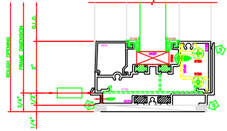
203 O.G. SILL SERIES: 403X - 2" X 4 1/2" SHEARBLOCK
