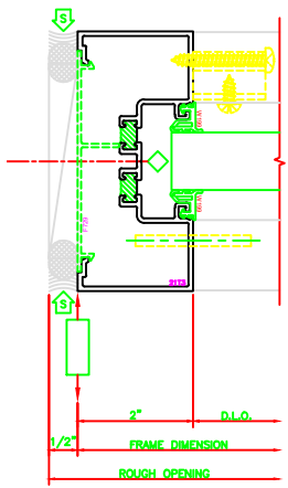
402 O.G. JAMB SERIES: 403X - 2" X 4 1/2" SHEARBLOCK
