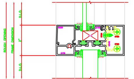
503 O.G. HORIZONTAL SERIES: 403X - 2" X 4 1/2" SHEARBLOCK
